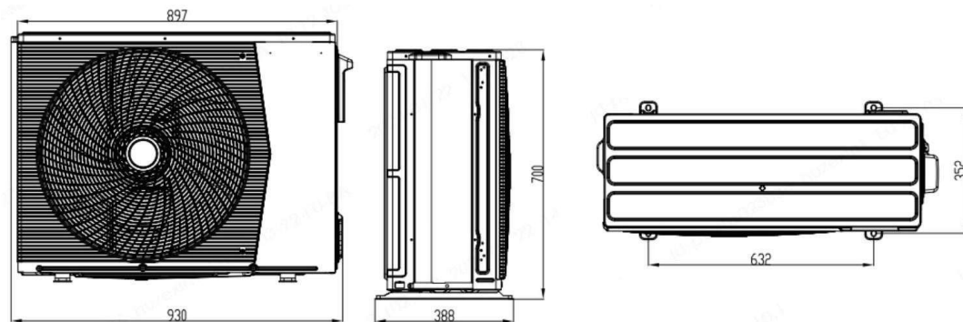
24K AUX-RAC-24TypeC/O
