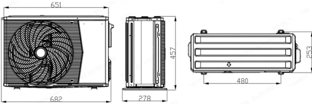
18K AUX-RAC-18TypeC/O
