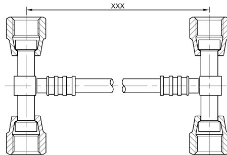
"T" with 2 Females 1/4 at 180° + "T" with 2 Females 1/4 at 180°
