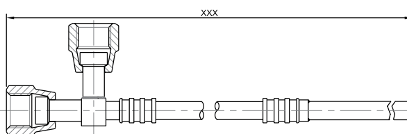
"T" With 2 Females 1/4 at 90° + Copper Brazing Tube
