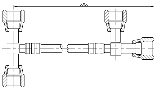
"T" with 2 Females 1/4 at 180° + "T" with 2 Females 1/4 at 90°
