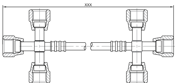
Cross with 3 Females 1/4 + Cross with 3 Females 1/4
