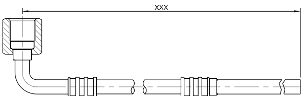
Elbow Female 1/4 + Copper brazing tube
