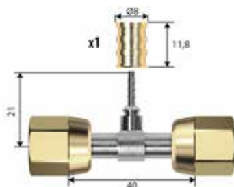
"T" Fitting With 2 Females 1/4 SAE At 180°
