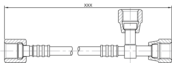
Straight Female 1/4 + "T" with 2 Females 1/4 at 90°
