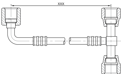
Elbow Female 1/4 + T With 2 Females 1/4 at 180°
