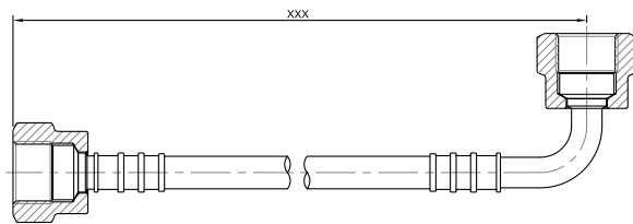
Straight Female 3/8 + Elbow Female 90° 3/8
