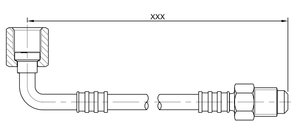
Elbow Female 1/4 + Male 1/4
