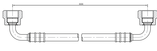
Elbow Female 90° 3/8 + Elbow Female 90° 3/8
