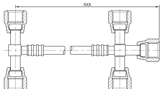
"T" with 2 Females 1/4 at 180° + Cross with 3 Females 1/4
