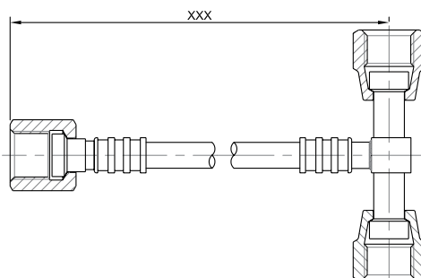
Straight Female 1/4 + "T" with 2 Females 1/4 at 180°
