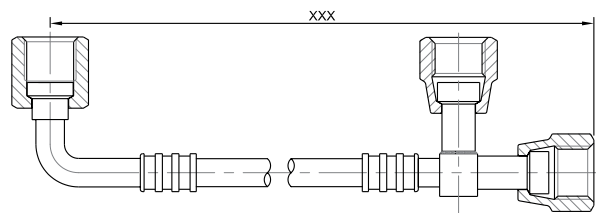
Elbow Female 1/4 + T With 2 Females 1/4 at 90°
