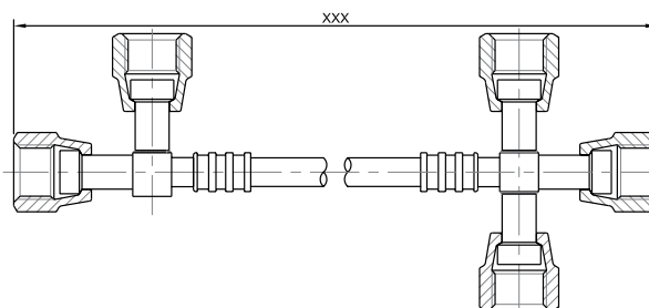
"T" With 2 Females 1/4 at 90° + Cross With 3 Females 1/4
