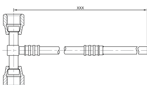
"T" With 2 Females 1/4 at 180° + Copper Brazing Tube
