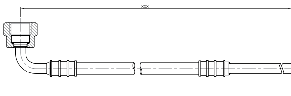
Elbow Female 90° 3/8 + Copper brazing tube
