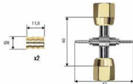
Cross Fitting With 2 Females 1/4 SAE At 180°
