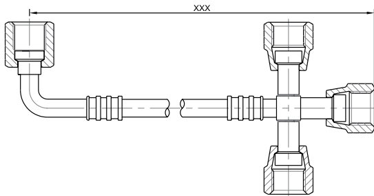
Elbow Female 1/4 + Cross with 3 Females 1/4
